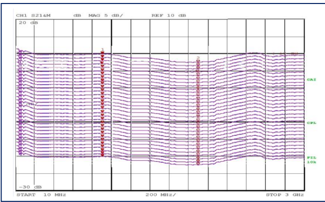
Gain vs. Tx Attenuation value: 0 to 31 dB in 1 dB step, 2.5 GHz RFoF for 'LNA Off' (similar behavior for 'LNA On')
