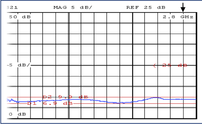
Gain vs. Freq. (S21), 2.5 GHz RFoF - 'LNA Off' (similar behavior for 'LNA On' with Gain higher by +29 dB)
