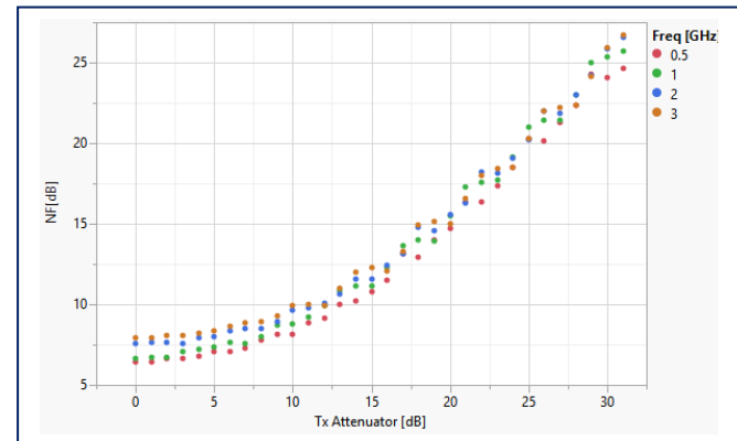
Noise Figure for 4 Freq. vs. Attenuator value, 2.5 GHz RFoF - 'LNA ON'
