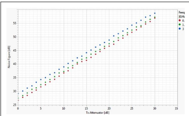
Noise Figure for 4 Freq. vs. Attenuator value, 2.5 GHz RFoF - 'LNA Off'
