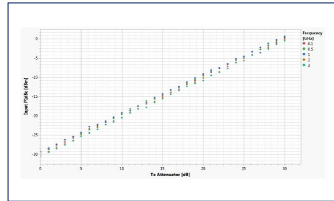
Input P1dBc at 5 frequencies, 2.5 GHz RFoF - 'LNA On'
