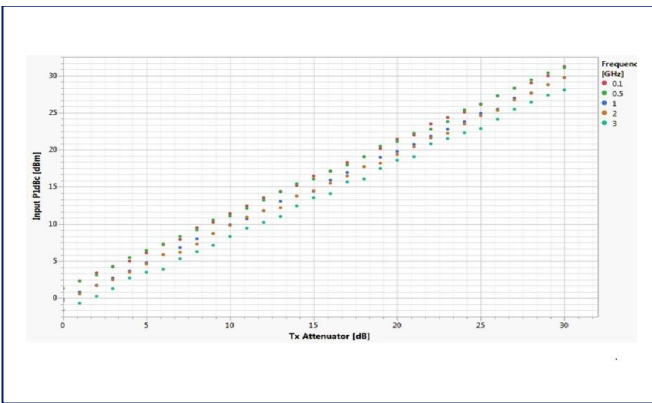
Input P1dBc at 5 frequencies, 2.5 GHz RFoF - 'LNA Off'
