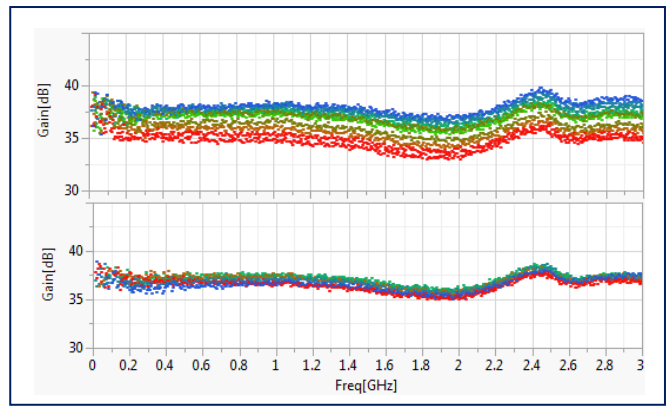
Gain Variation over Temperature for -20 °C (blue) to +70 °C (red), 'LNA On' without compensation (top). With Compensation (bottom). Similar behavior for Gain Variation over Temperature for 'LNA Off'.
